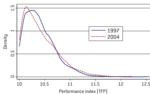
Figure 4: Introduction of the euro and changes in firm-level productivity distributions, machinery industry in Italy
