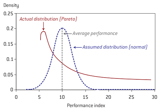
Figure 1: Pareto versus normal distributions
